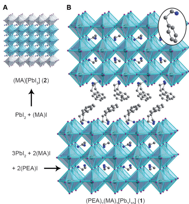
Figure 1. A) Crystal structures of the 3D perovskite (\text{MA})[\text{PbI}_3] ( 2 , from Ref. [12a]) and B) the 2D perovskite (\text{PEA})_2(\text{MA})_2[\text{Pb}_3\text{I}_{10}] ( 1 ). The inorganic layers in 1 can be structurally derived from 2 by slicing along specific crystallographic planes (turquoise sheets in (A)). Inset: a PEA cation in the organic layers. Atom colors: Pb = turquoise; I = purple; N = blue; C = gray. Disordered atoms and hydrogens omitted for clarity.
