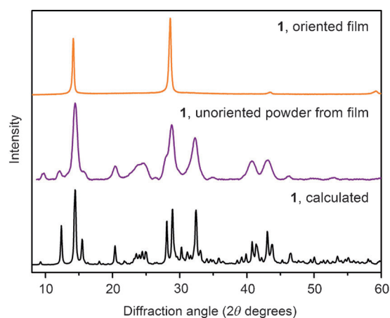
Figure 2. Powder X-ray diffraction (PXRD) patterns of (\text{PEA})_2(\text{MA})_2[\text{Pb}_3\text{I}_{10}] ( 1 ) as an oriented film (top) and as powder scraped from a film and measured in a glass capillary (middle), and the calculated PXRD pattern from the single-crystal X-ray structure of 1 (bottom).
